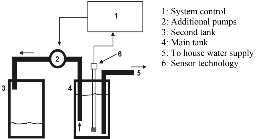
Diagram 14: Plant layout example
